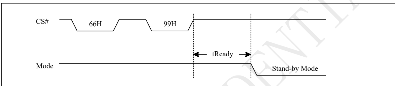
Figure 10-51b Reset Sequence
