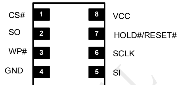
8-Pad USON (1.5x1.5mm/3x2mm)
